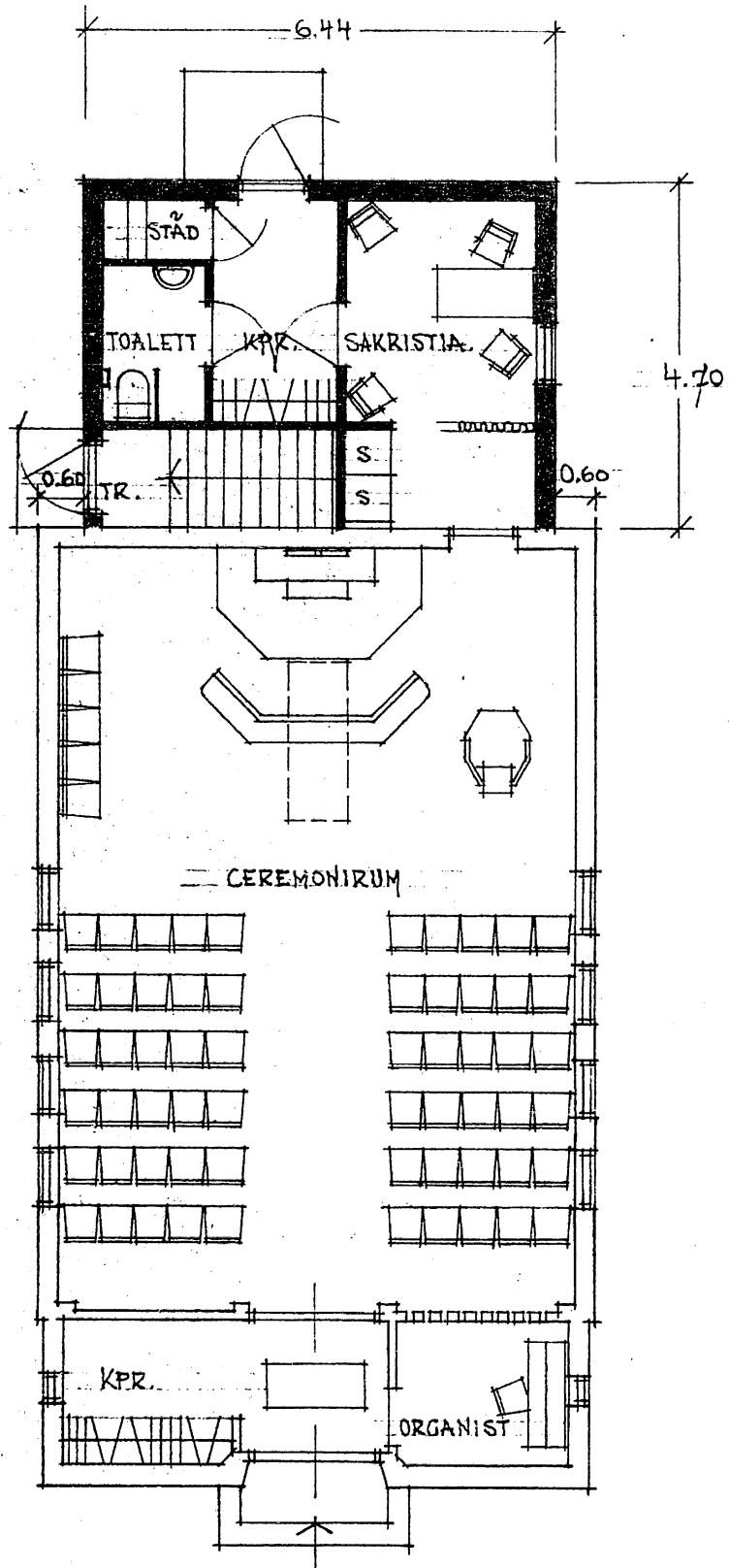
BOTTENPLAN
